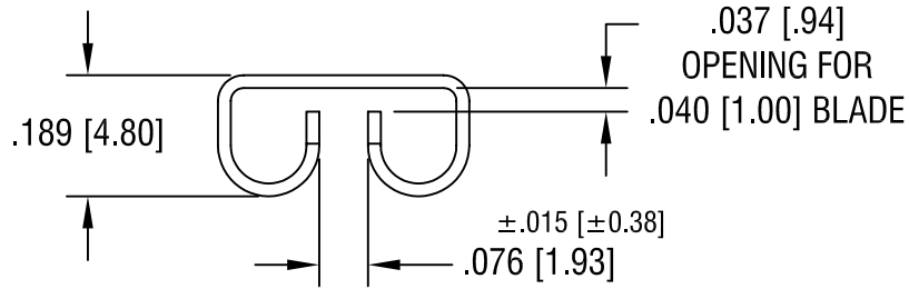
MOUNTING DETAIL
