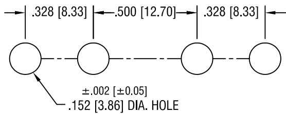
MOUNTING DETAIL
