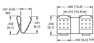
MATERIAL: .010 (.25) Spring Steel, Nickel Plate
