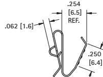
MATERIAL: 012 (.30) Spring Steel, Nickel Plate
