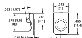
MATERIAL: 010 (.25) Spring Steel, Nickel Plate
