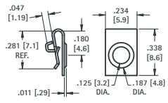
MATERIAL: .010 (.25) Spring Steel, Nickel Plate
