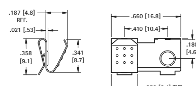
MATERIAL: .010 (.25) Spring Steel, Nickel Plate
